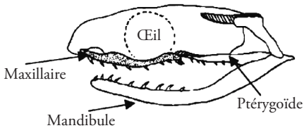
Figure 9 Denture des serpents
