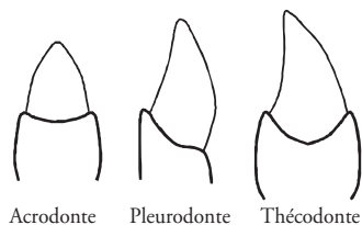
Figure 3 Dispositions dentaires de reptiles
