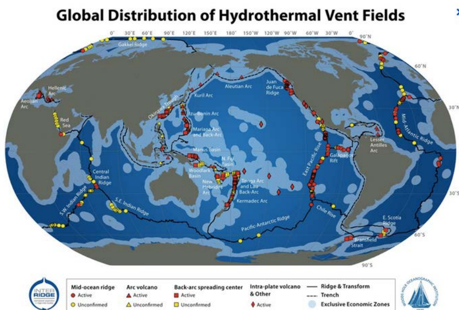
Figure 8 – Distribution des sources hydrothermales (Source : Hein et al. 2013)
