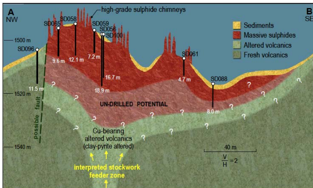
Figure 3 — Mineral Resource Estimate, Solwara 1 Project, Bismarck Sea, Papua New Guinea. (Source : De Lipton, I, 2008 1 ).
