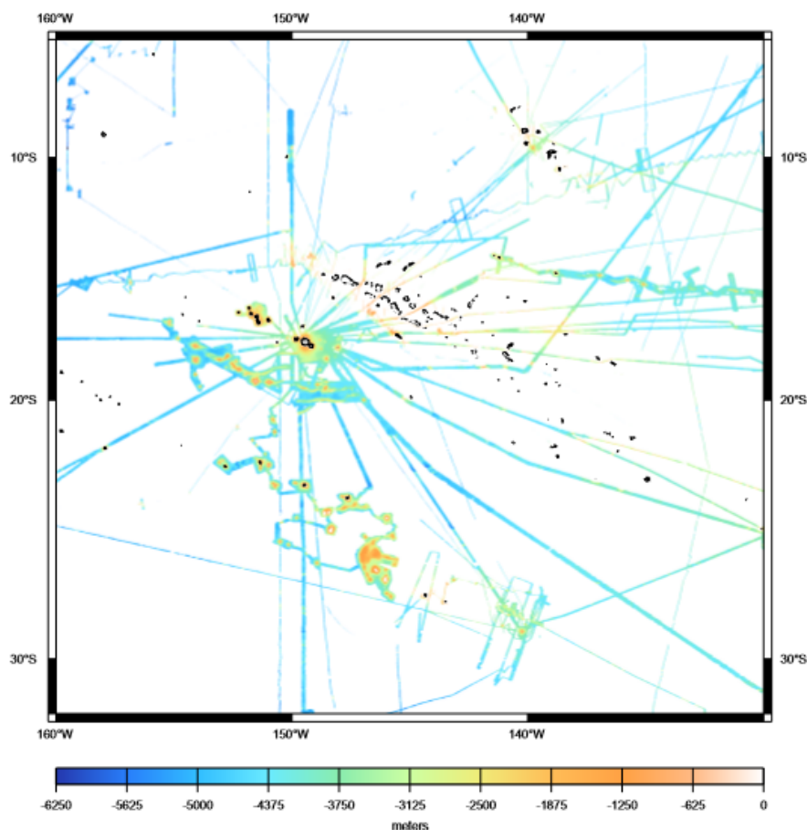
Figure 2 – New depth compilation for French Polynesia. Gaps between soundings have been left blank (Source: Jordahl et al., 2004)
